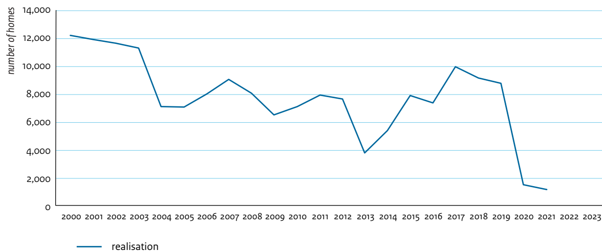
Figure 3.2 Development of the number of houses with a noise exposure of 58 dB(A) L_{den} or more
