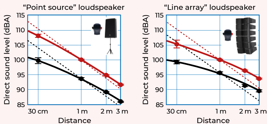
Figure A10.1: Direct sound levels close to point source and line array loudspeakers
