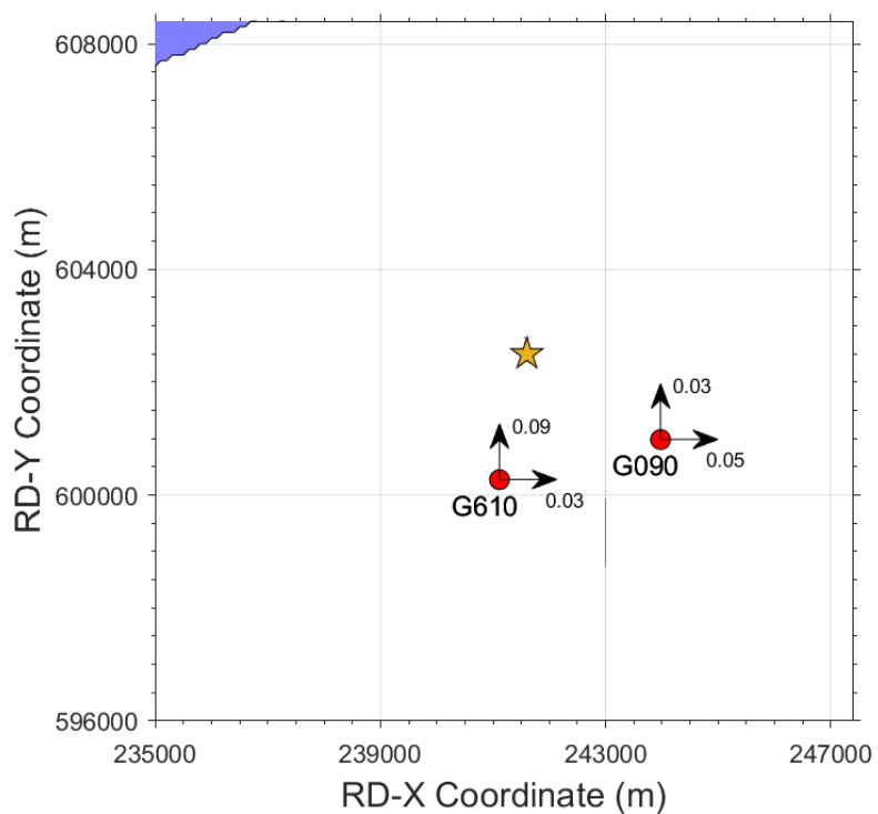
Figure 3.11 Horizontal components of PGA (upper) and PGV (lower) recorded during event 39 ( M_L 1.7 ) at epicentral distances of less than 6 km; units are \text{cm/s}^2 and \text{cm/s} , respectively.
