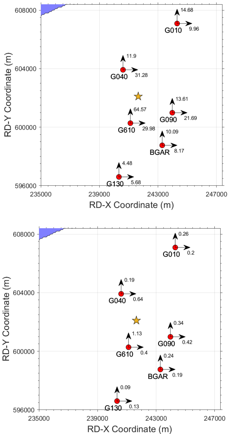
Figure 3.10 Horizontal components of PGA (upper) and PGV (lower) recorded during event 38 ( M_L 2.7 ) at epicentral distances of less than 6 km; units are cm/s^2 and cm/s , respectively.
