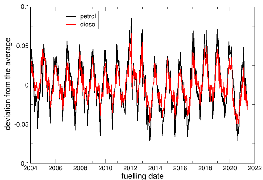
Figure 8-1: The seasonal changes in fuel consumption on a fleet level. For every individual vehicle in the Travelcard fleet the time dependent deviation from its long-term average fuel consumption was calculated, and averaged.
