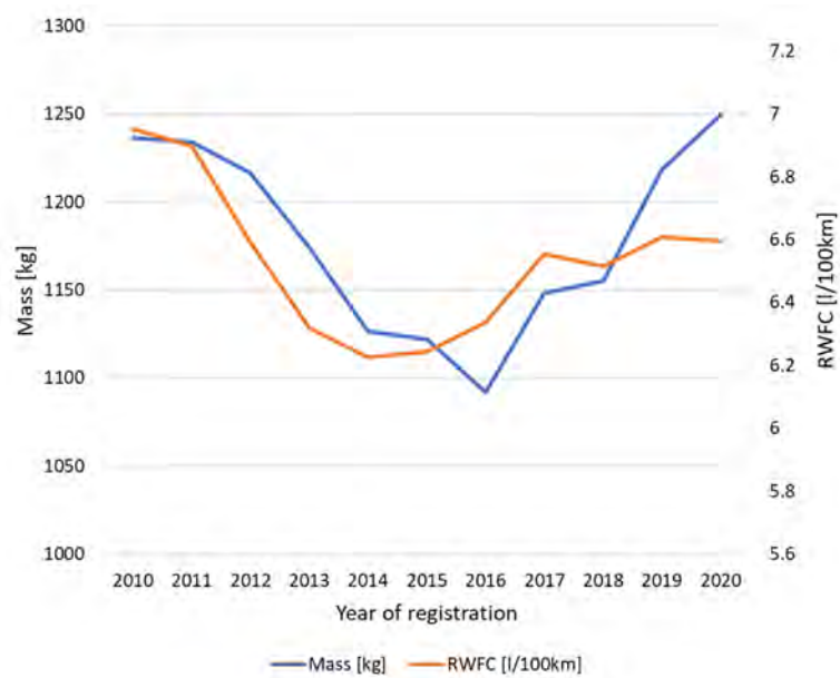
Figure 3-1: Trend of average vehicle mass and real-world fuel consumption per registration year for petrol passenger cars (incl. hybrids, excl. plug-in hybrids).
