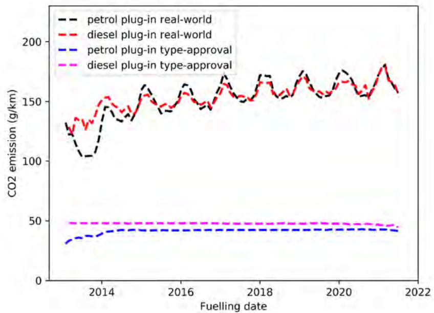
Figure 2-5: Average real-world and NEDC type approval tailpipe CO 2 emissions of all plug-in hybrid petrol and diesel vehicles in the database.
