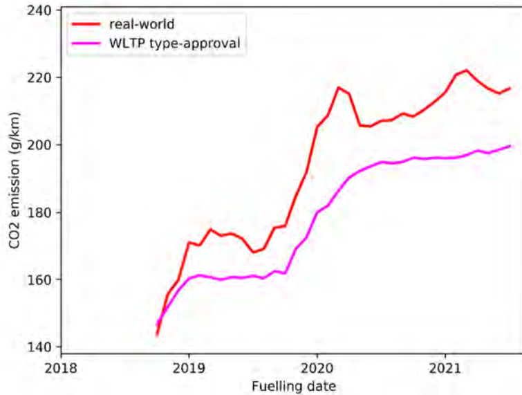
Figure 6-2: Average real-world and type approval CO 2 emissions of light commercial vehicles in the Travelcard fleet that were WLTP type approved. The number of vehicles was limited at the start of the lines.
