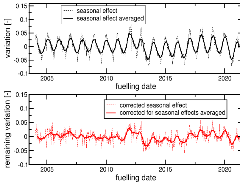
Figure 7-4: After the correction for impacts of daily mean temperature, average wind speed, and irradiation, some seasonal effects in the fuel consumption of petrol cars remain, especially for the years after 2016..
