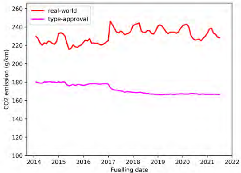
Figure 6-3 Average real-world and NEDC-based type approval CO 2 emission of all light commercial vehicles in the Travelcard fleet. The number of vehicles was limited at the start of the lines.
