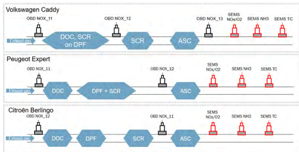
Figure 4.1: Schematic overview of the position of catalysts, in-vehicle NO x sensors and installed SEMS sensors (in red) in the exhaust pipes of the three tested Euro 6d diesel vehicles. For each vehicle the in-vehicle NO x sensors (named 'OBD NOX_1x') have a different position in the exhaust pipe. Only the in-vehicle NO x sensor ('OBD NOX_13') of the Volkswagen Caddy is measuring actual tailpipe-out NO x emissions.
