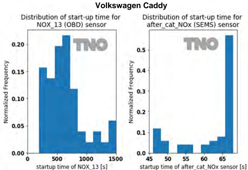
Figure 4.2: Monitoring data of the Euro 6d Volkswagen Caddy. On the left: distribution of start-up times of the in-vehicle NO x (tailpipe-out). On the right: distribution of start-up times for the SEMS NO x sensor.
