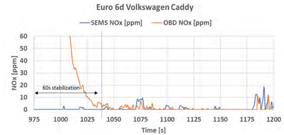
Figure 4.3: Stabilization time after activation of the OBD NO x sensor of the Euro 6d Volkswagen Caddy.
