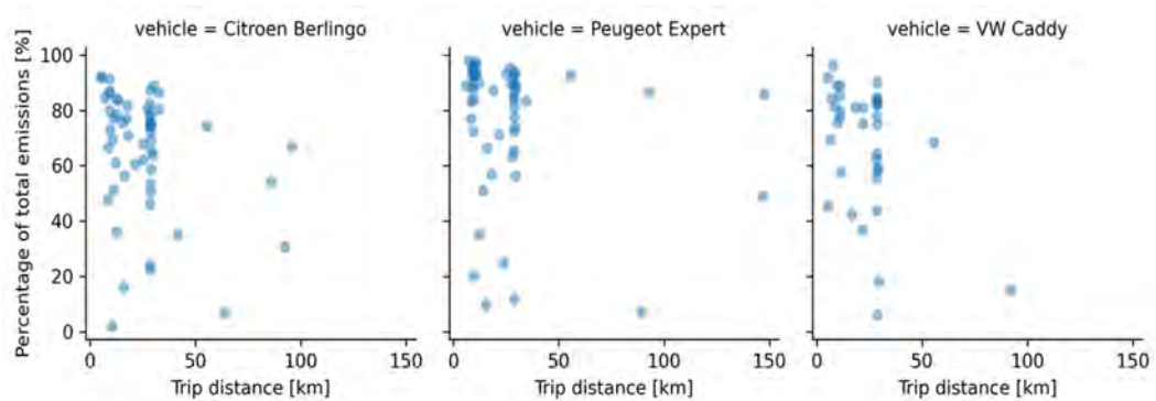
Figure 3.4: Cold start \text{NO}_x emission of three Euro 6d diesel vehicles as a percentage of the total trip emission as a function of trip distance. Each dot represents a single cold start trip.
