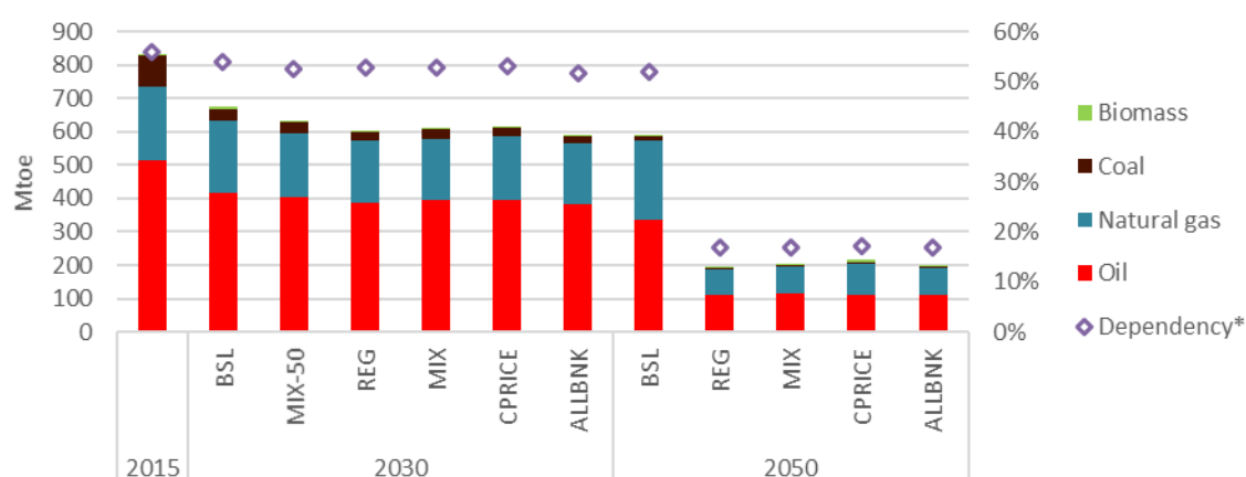
Figure 12: Energy imports
