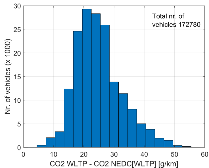
Figure 5-7: The distribution of differences over all WLTP registrations, show a large spread. The difference is 25 g/km, but the normal spread is also 25 g/km with a full range between 5 and 50 g/km.
