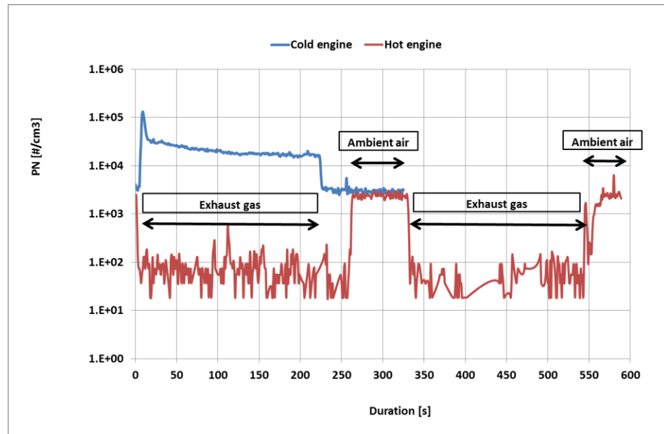
Figure 35 PN emissions of a euro 6 diesel vehicle with DPF at cold and hot engine operation.
