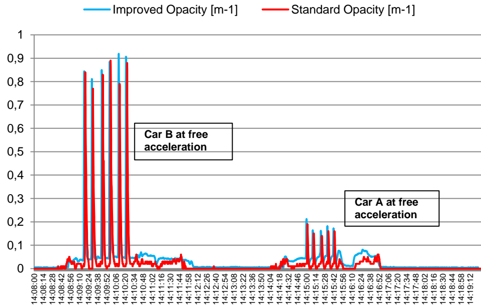
Figure 32 Results of opacity measurement of two cars with high smoke values, using the standard opacity meter and the improved opacity meter, both in the filtered mode.
