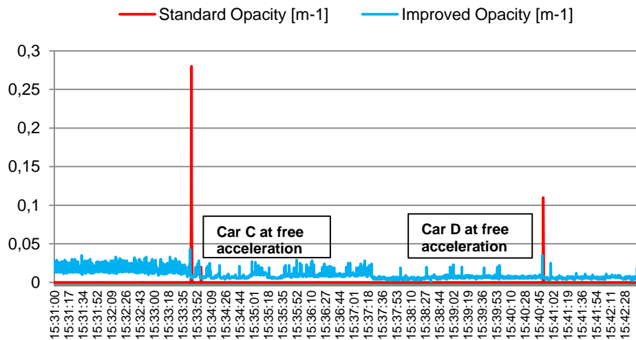
Figure 33 Results of opacity measurement of two cars with low smoke values, using the standard opacity meter and the improved opacity meter, both in the unfiltered mode.
