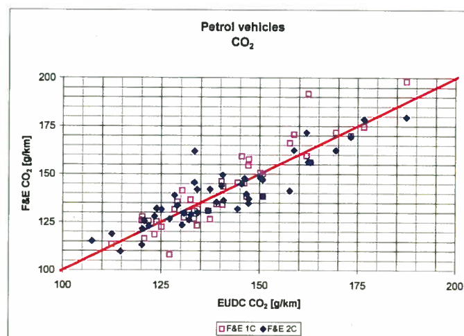
Figure 37 CO 2 -emission of EUDC TA driving cycle versus E&C driving cycles
