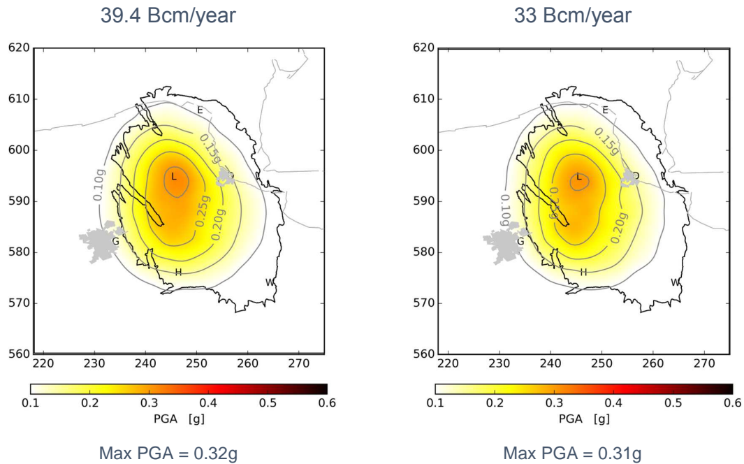
Figure C1 Mean hazard map for period 1-1-2015 to 1-1-2017. Production: 39.4 Bcm/year and 33 bcm/year. Compaction Model: Inversion, Activity Rate: V1, M \geq 3.5 Metric shown is 0.2% year -1 chance of exceedance (10% chance in 50 years).
