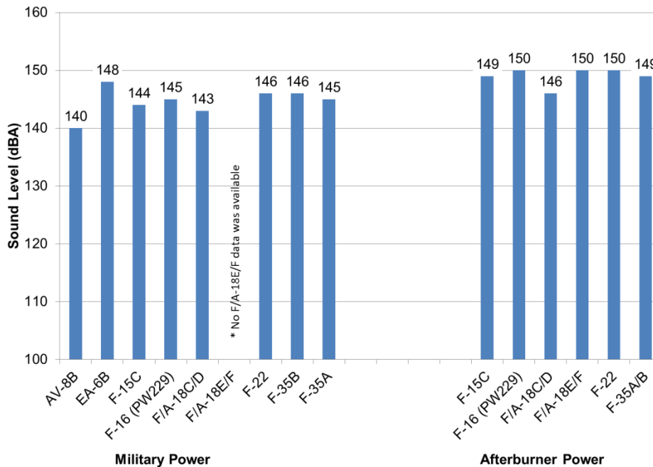
Aircraft Ground Noise Figure 1
