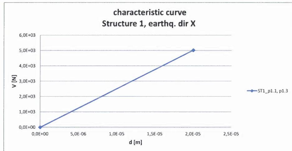
Figure 6.6. Floor characteristic V-d curve structure 1; x-direction
