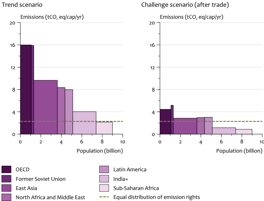
Per-capita emissions in 2040, and emission caps based on equal per-capita distribution on an emissions convergence path to 2050 (reaching 2 °C target). Analyses: TIMER/FAIR
